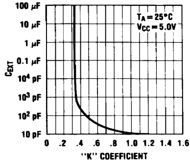
FIGURE 6. Typical "K" Coefficient Variation vs Timing Capacitance
