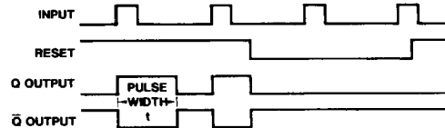
TL/F/6611-11
