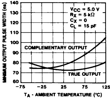
FIGURE 5. Minimum Output Pulse Width vs Ambient Temperature
